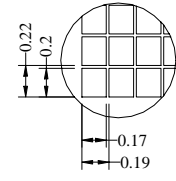
Detail "A" Scale (10:1)
