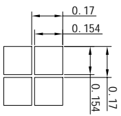
Detail A (20:1)
